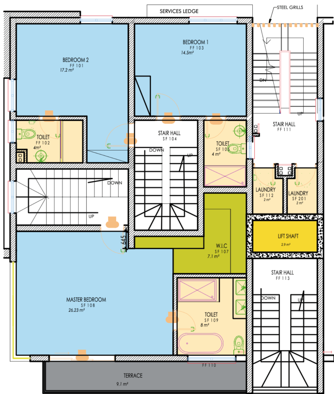
3 Bedroom Maisonette Second Floor Plan
