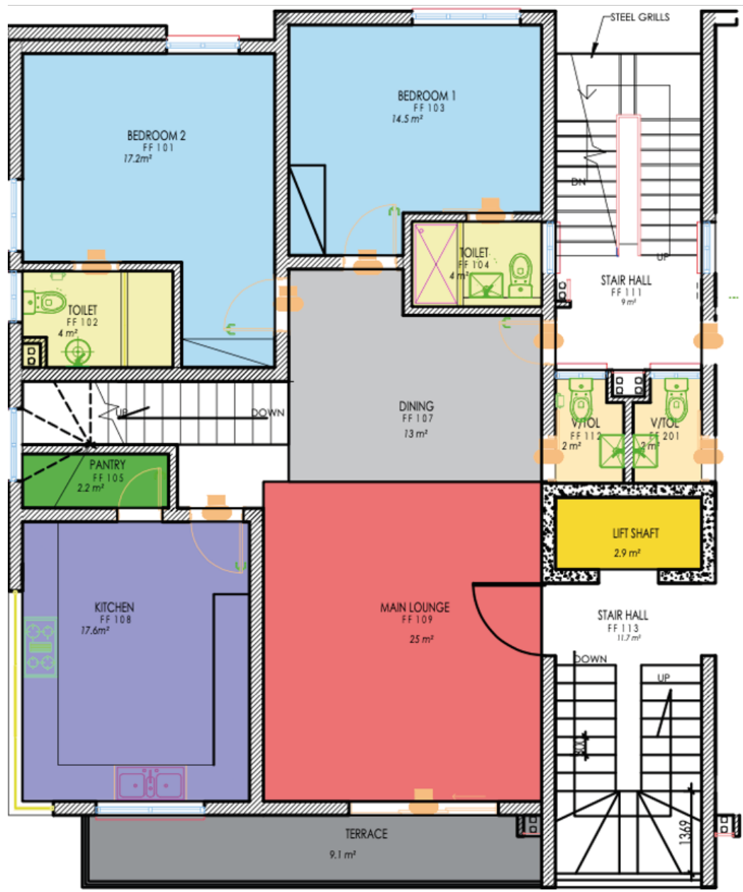
3 Bedroom Maisonette First Floor Plan
