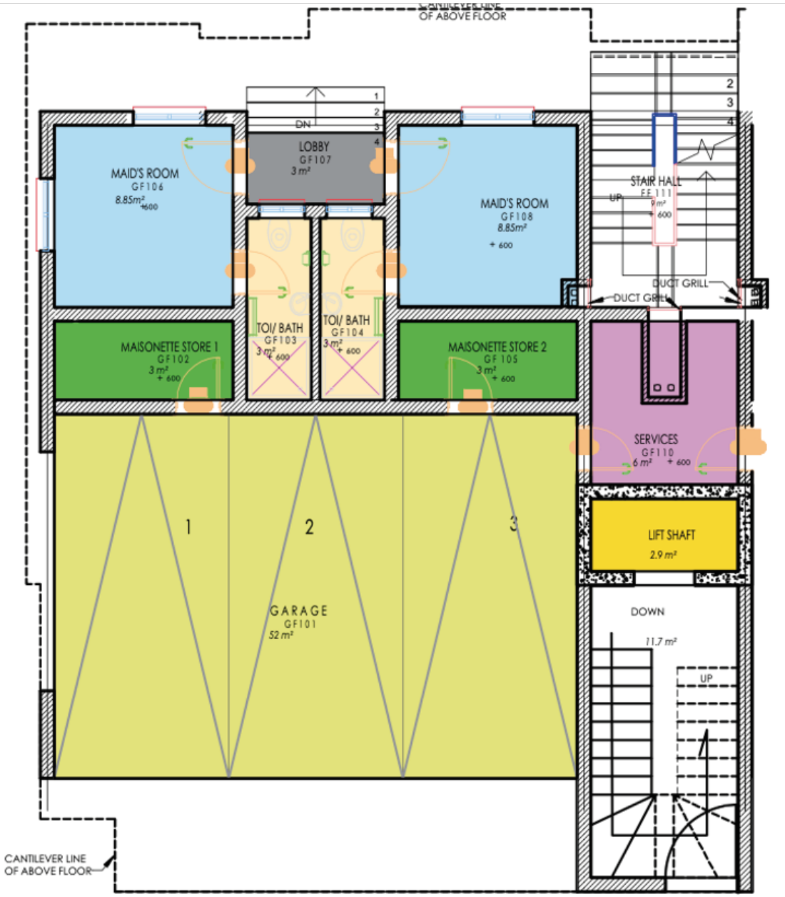
3 Bedroom Maisonette Ground Floor Plan
